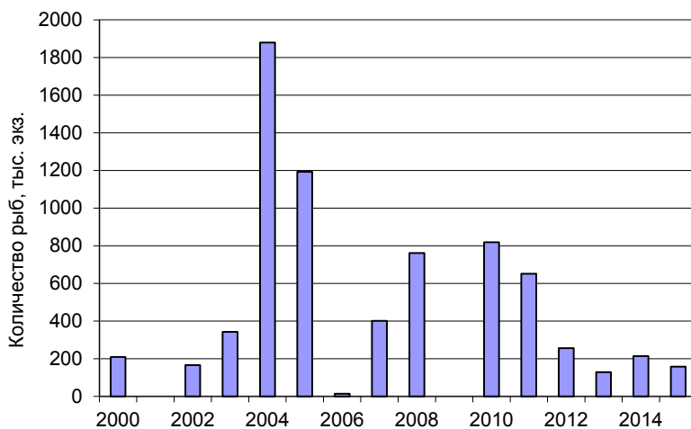
Fig. 1. Number of masu juveniles released from the hatcheries of Sakhalin Region
